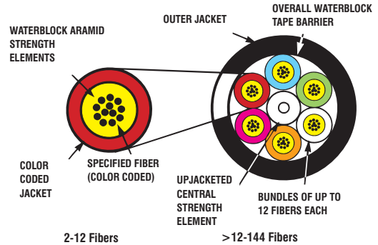
FIBER BUNDLE DETAIL
